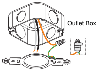
Ground wire from mounting bracket Green ground screw Ground wire from supply
